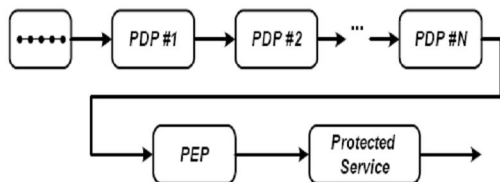
Figure.5 Sequential decision making pattern
