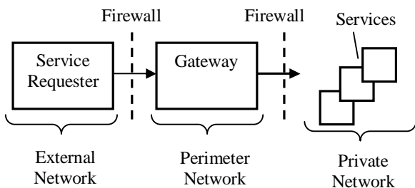
Figure.3 Gateway Pattern
