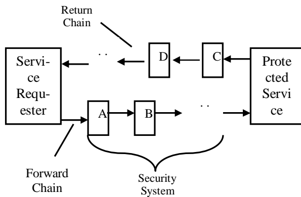
Figure.1 Service Chains
